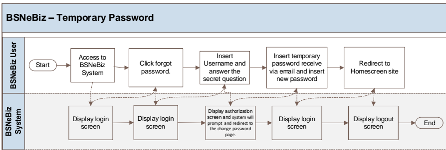
Diagram 7: Temporary Password flow
