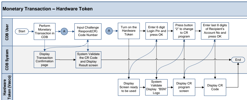
Diagram 1: Hardware Token Flow Diagram
