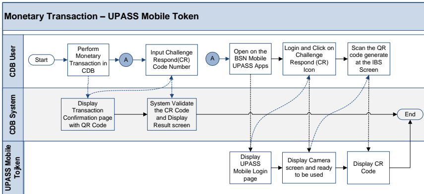
Diagram 2: Mobile Token Flow Diagram
