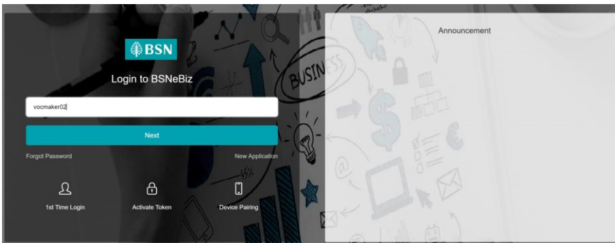
Figure 9: Login Screen
