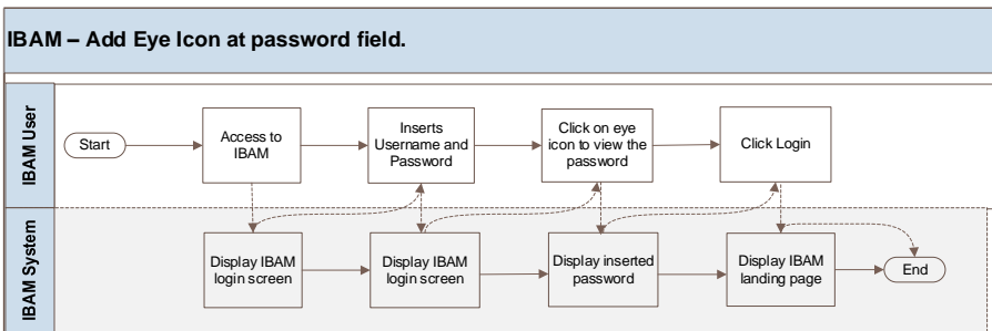
Diagram 4: IBAM Login Flow
