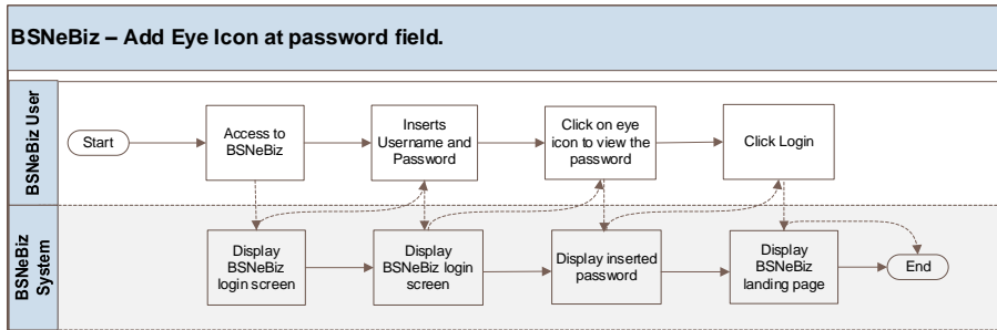
Diagram 5: BSNeBiz Web Eye Icon
