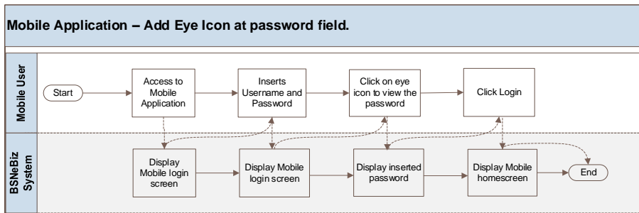
Diagram 6: Mobile Application Eye Icon flow
